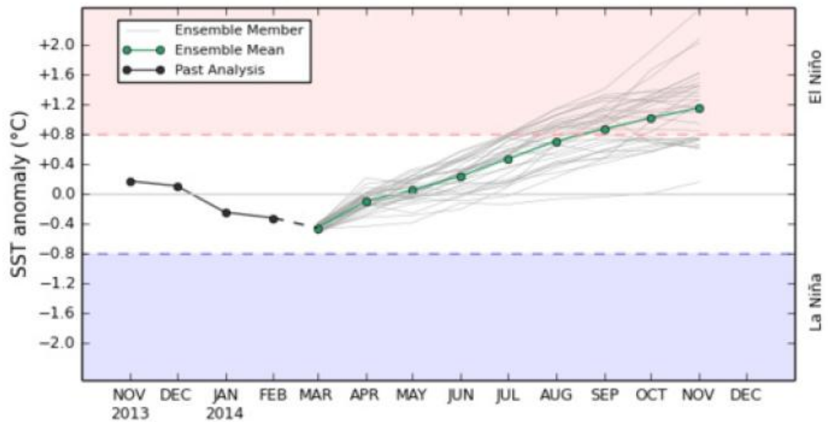
POAMA monthly mean NINO34 - Forecast Start: 2 MAR 2014
