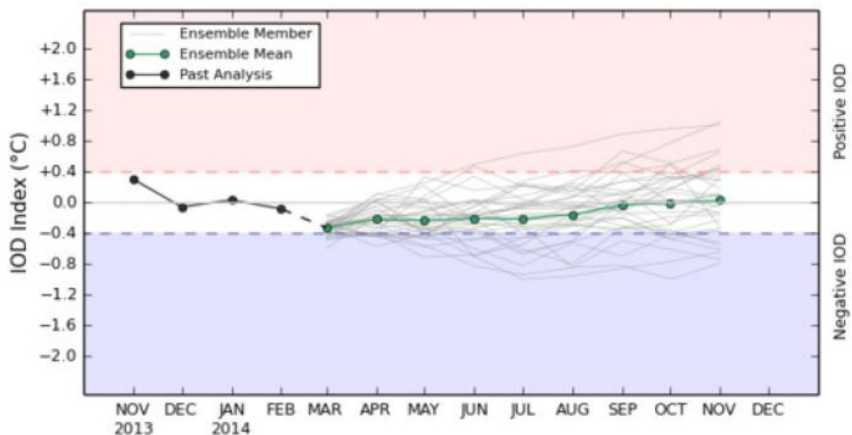
POAMA monthly mean IOD - Forecast Start: 2 MAR 2014
